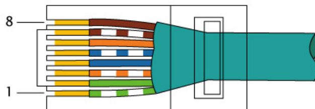
EIA/TIA-568A
